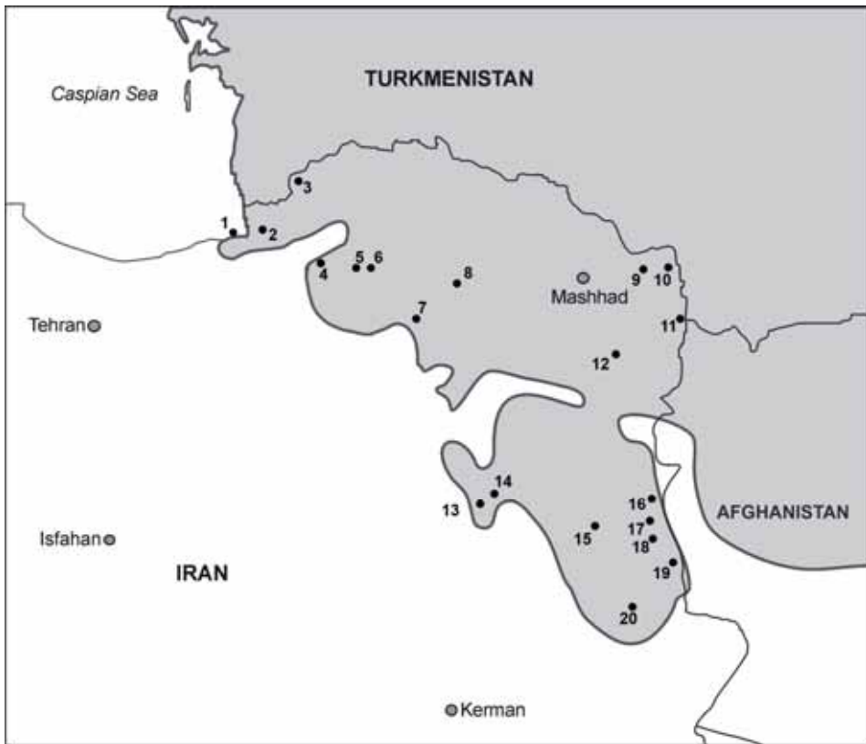
Fig. 1. Localities of records and range of Agrionemys horsfieldii in Iran. The range of the species in Iran and beyond is shown in grey. Own data, unless otherwise stated. – 1 - Miankaleh Peninsula 12 km W of Bandar-e-Turkmen, 36°54'N, 54°02'E, 20 m a.s.l. (KAMI 2005); 2 - Near Gorgan 36°50'N, 54°26'E (KAMI 1999); 3 - Gonbad Kavous, banks of the Atrak river (KAMI 1999); 4 - Khoshyeilagh Wildlife Refuge 36°36' to 37°02'N and 55°11' to 55°53'E, 1200 m a.s.l. (KAMI 1999); 5 - 85 km E of Shahrud, near Miyandasht, 36°25'N, 55°54'E, 1177 m a.s.l.; 6 - 115 km E of Shahrud, near Abbas Abad, 36°21'N, 56°17'E, 1270 m a.s.l.; 7 - Kalateh-rey sand dunes, 16 km NW of Zamanabad, 35°41'N, 56°38'E, 1060 m a.s.l. (CAS 228637); 8 - Sandy foothills near Sabzevar, 36°12' N, 57°30'E (KAMI 1999); 9 - East Kopetdag, 3 km NE of Mazdavand, 36°09'N, 60°35'E, 940 m a.s.l.; 10 - 13 km SW Sarakhs 36°32'N, 61°11'E (MMTT; ANDERSON 1979); 11 - Kuh-e Shakhneshin Mts, 25 km SW of Saleh Abad, 35°30'N, 60°50'E, 1690 m a.s.l.; 12 - Kuh-e Sorkh Mts, 35 km E of Dowlat Abad, 35°20'N, 59°54'E, 1830 m a.s.l.; 13 - Eshdeger range, foothills near Deyhuk, 33°15'N, 57°27'E, 1546 m a.s.l. ; 14 - Kuhistan [region centering 33°N, 57°E] (WERNER 1936); 15 - Qayen Mts, 7.2 km N of Sarbisheh, 32°39', 59°46'E, 1855 m a.s.l. (CAS 228669); 16 - Qayen Mts, Ahangarun, between Ahangarun and Doroh, 33°25'N, 60°13'E (ZARUDNOI 1903, ANDERSON 1979); 17 - Qayen Mts, near Gazik, between Ahangarun and Doroh, 32°60'N, 60°13'E (ZARUDNOI 1903); 18 - Qayen Mts, near Tabas, between Ahangarun and Doroh, 32°48'N, 60°14'E (ZARUDNOI 1903); 19 - Qayen Mts, Rud-i-Mil, between Chah-i-Sagak and Doroh, 32°17'N, 60°30'E (GRAY 1873, ANDERSON 1979); 20 - Qayen Mts, 40 km NW of Nehdandan, 31°51'N, 59°46'E., 1750 m a.s.l.; – Additional localities: Kara-iltschi Mts (NIKOLSKY 1897); Tauran (WERNER 1936); Almelh, Chodech 'Abbas, Mohammad Reza Shah National Park (MMTT).
